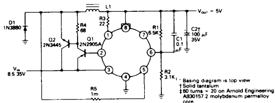
4A Switching Regulator
