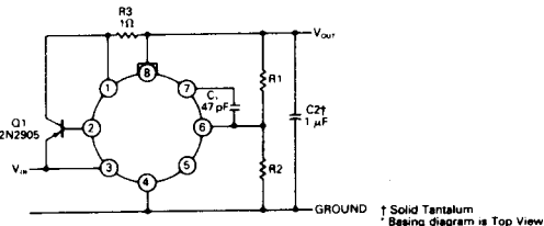
200 mA Regulator
